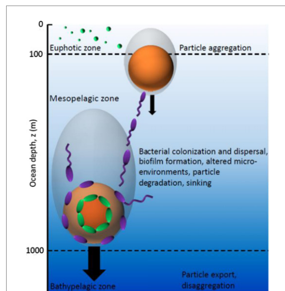
Figure 7. Organic particles, formed by the aggregation of fragments of decaying organisms, leave the euphotic zone, sink through the mesopelagic zone at a size-dependent rate, and are altered as they sink by bacterial activity. Cells adopt a variety of foraging strategies, including irreversible attachment to the particle surface with formation of biofilm (green cells), or a flexible strategy involving repeated colonization and dispersal [62] (violet cells). These processes regulate the biological pump, the process by which particulate carbon sinks and reaches the bathypelagic zone to be sequestered in the ocean depths for thousands of years.
