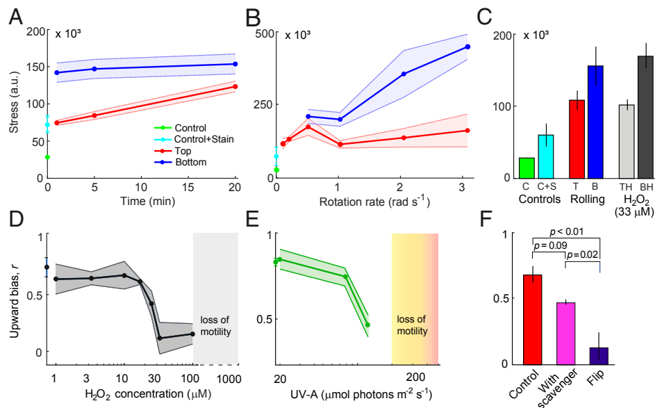
Fig. 2. Bistability in oxidative stress mediates vertical migration of H. akashiwo . Oxidative stress level, caused by intracellular ROS accumulation, is shown as a function of (A) the time exposed to rolling ( \Omega = 1 \text{ rad} \cdot \text{s}^{-1} ) and (B) the rotation rate (rolling time t = 5 \text{ min} ). Curves show the increase in oxidative stress levels for the top (red, “Top”) and the bottom (blue, “Bottom”) subpopulations. Also shown are the baseline fluorescence signal of untreated control cells (green, “Control”) and of control cells treated with the fluorescent stain CM-H 2 DCFDA, a general oxidative stress indicator (cyan, “Control+Stain”). Stress levels were computed from flow cytometric measurements (mean \pm SD of at least three replicates). (C) Oxidative stress level caused by intracellular ROS accumulation after exposure to exogenous H 2 O 2 or to 20 min of rolling ( \Omega = 1 \text{ rad} \cdot \text{s}^{-1} ). Controls (same as in A and B) are shown in green and cyan. Bars show the oxidative stress levels for the top (red, “T” for rolling; light gray, “TH” for H 2 O 2 ) and the bottom (blue, “B” for rolling; dark gray, “BH” for H 2 O 2 ). Stress levels (a.u., arbitrary units) were computed from flow cytometric measurements (mean \pm SD of three replicates). Cells that switch to downward-swimming behavior show elevated stress levels (“B” and “BH”), while cells that continue to swim upwards (“T” and “TH”) show stress levels closer to those of the controls. (D) Upward bias as a function of the concentration of H 2 O 2 added to the medium 30 min before measurements. H 2 O 2 concentrations above 15 \mu\text{M} elicit the population split in migration direction. Above 100 \mu\text{M} H 2 O 2 , cells lost motility (SI Appendix, Fig. S12B). (E) Upward bias as a function of the intensity of UV-A light (emission peak = 395 nm) applied for 30 min. Photon flux densities above 80 \mu\text{mol photons m}^{-2} \cdot \text{s}^{-1} elicit the population split in migration direction. Above 200 \mu\text{mol photons m}^{-2} \cdot \text{s}^{-1} , cells lost motility (SI Appendix, Fig. S12C). (F) Upward bias for cells kept in still conditions (red bar, “Control”), for cells that were flipped (blue bar, 100 flips, \Omega = 1 \text{ rad} \cdot \text{s}^{-1} , \tau_{\text{W}} = 0 \text{ s} ), and for cells that were flipped after having been cultured in the presence of a scavenger of ROS (100 \mu\text{M} KI, magenta). Populations differed significantly in upward bias (one-way ANOVA, F_{2,7} = 19.8 , P = 0.001 ). Brackets show P values from post hoc Tukey’s honest significant difference (HSD) tests (SI Appendix, Table S1). For all panels, data shown correspond to mean \pm SD of three replicates.
